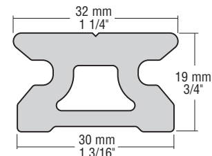
R32 Big Boat traveler track
