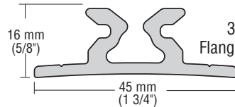
2720 Small Boat traveler track
